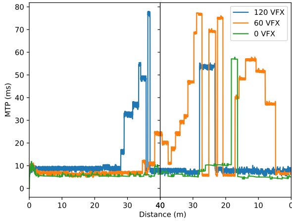
Fig. 8: Behaviour of the Motion-to-Photon latency (MTP) in milliseconds for the remote rendering experiment with Oculus AirLink.
